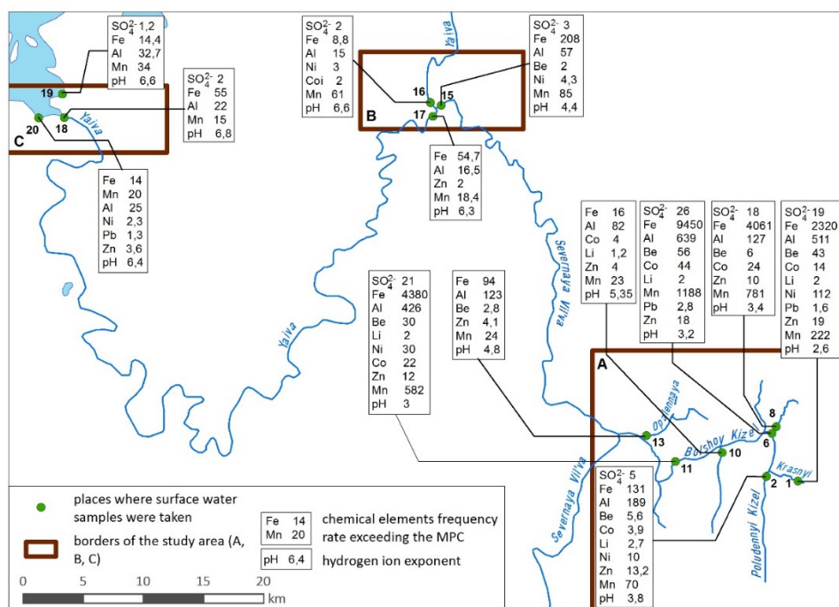
Figure 3. The Schema of monitoring sections location after the mines closure in the Yaiva basin.
